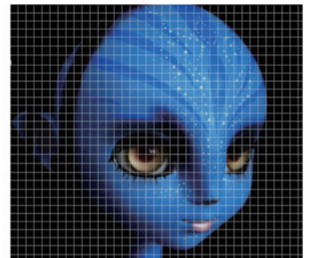
H.264 compression
